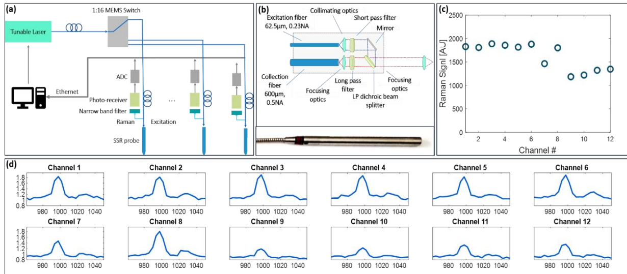
Fig.1 (a) Illustration of a multiplexed Swept-Source Raman network. (b) Image of the custom multimode probe we had designed and used to acquire the spectra with the internal optical components. (c) Comparison of the Raman signal power of 12 of 16 switch channels. (d) Spectra of polystyrene collected with 80mW, 2 sec integration time with 23 data points using the multimode probe through 12 of the 16 channels of the datacom switch. All 16 ports are functional and the in signal is dominated by variability in the probe to sample alignment.
